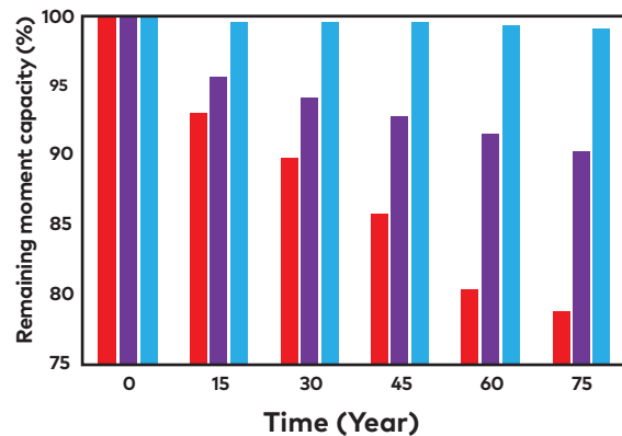
Percentage of drop in the moment capacity as a function of age.
