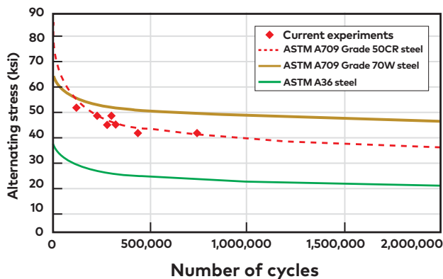
Fatigue behavior ASTMA709 Grade 50CR steel in comparison to the other conventional structural steels (1 ksi = 6.9 MPa).
